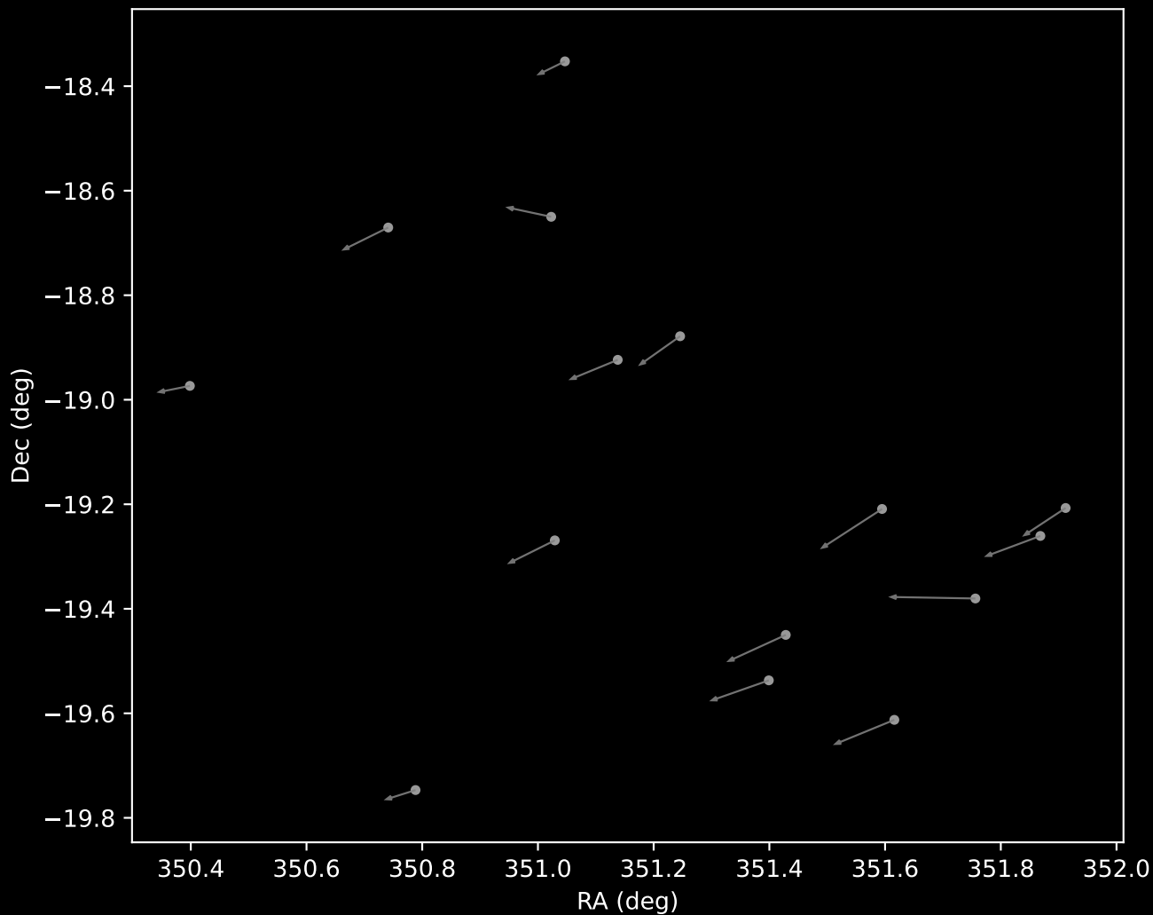
APOGEE DR17 Cluster 14 Proper Motion Vectors (n=15)
