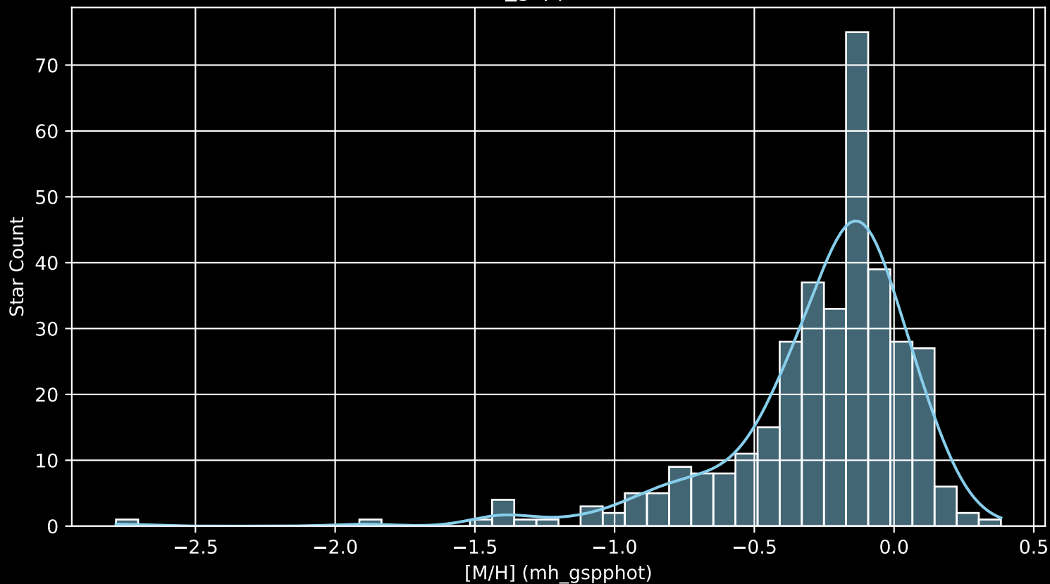
APOGEE DR17 Field: [000+17] [M/H] (mh_gspphot) (n= 351)
