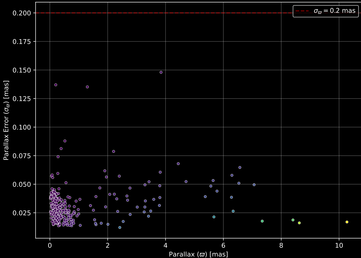
APOGEE DR17 Field: [000+17] Parallax Quality (n= 354)
