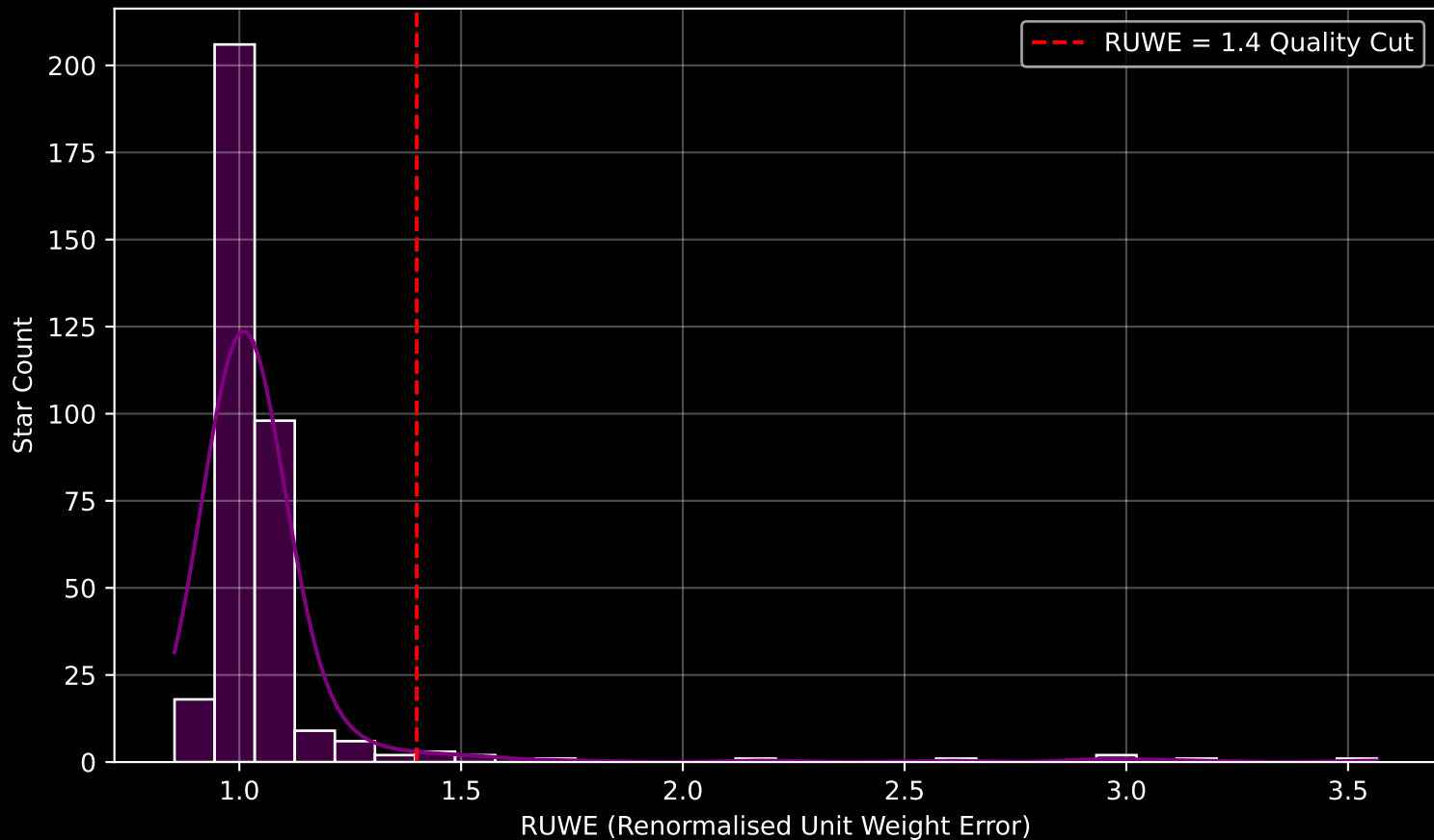
GAPOGEE DR17 Field [000+17] RUWE Distribution (n= 351)
