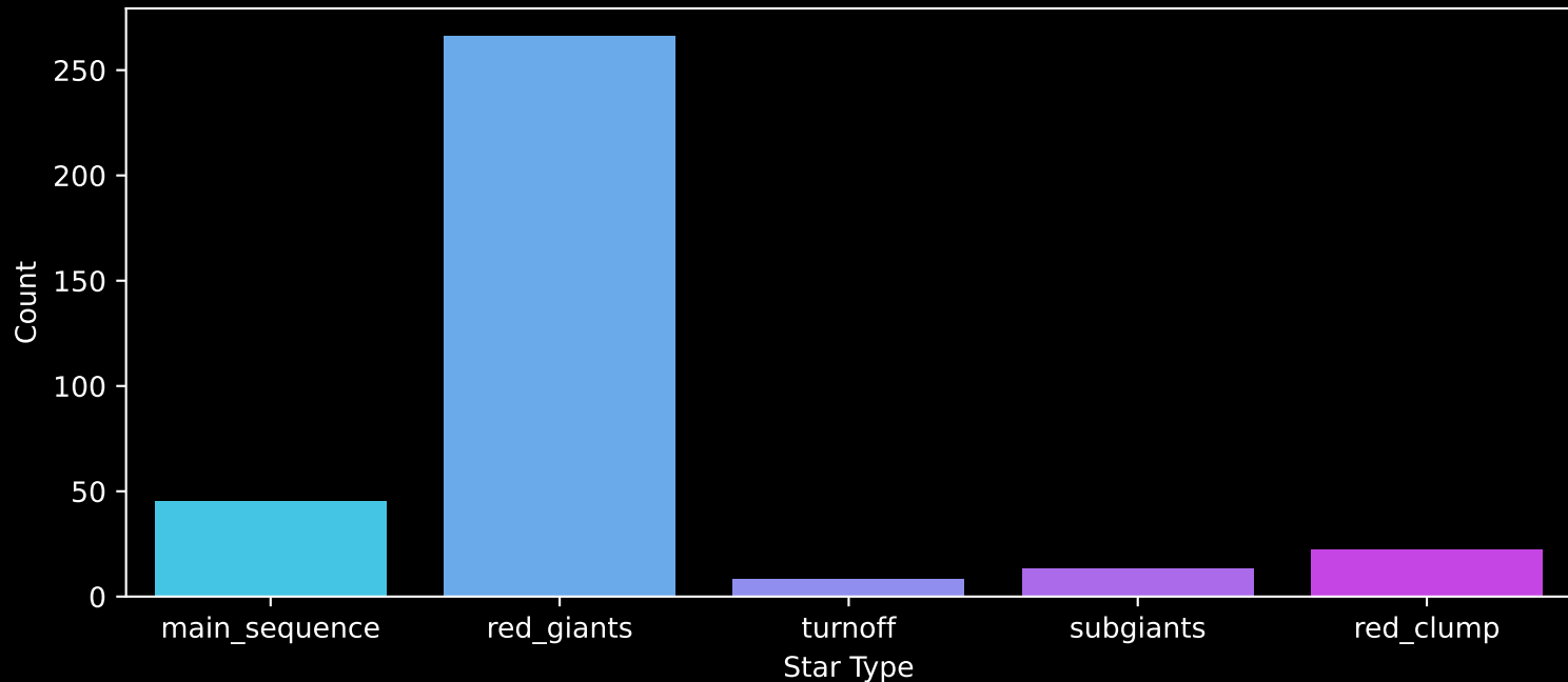
APOGEE DR17 Field: [000+17] Count plot of Star Type
