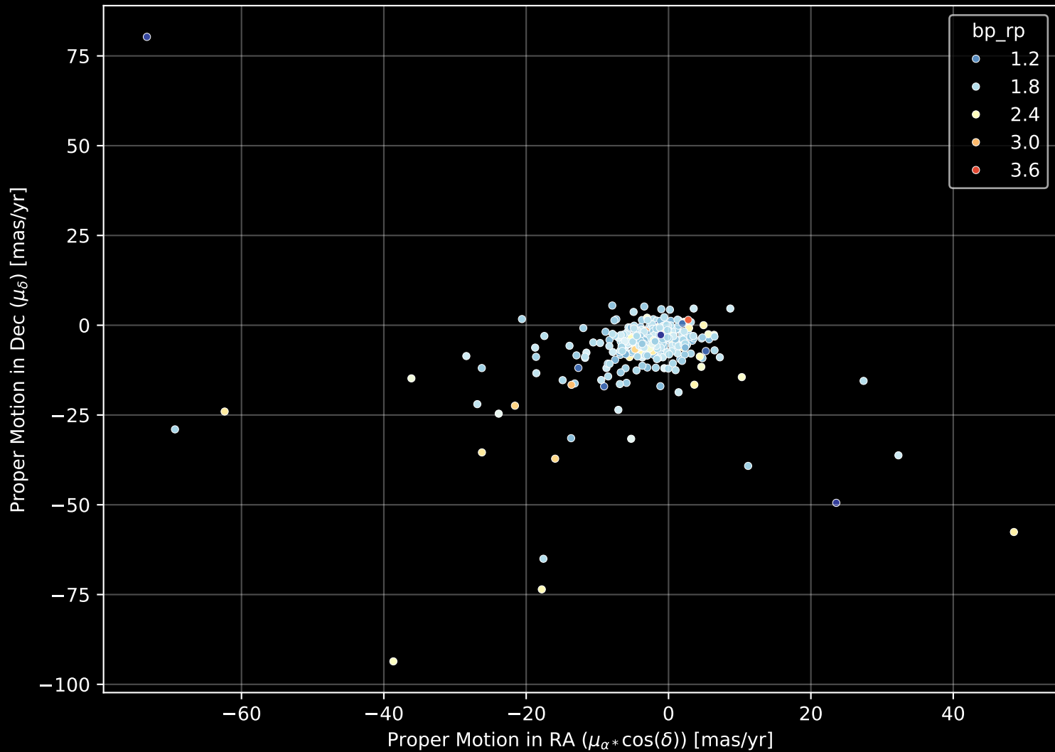
APOGEE DR17 Field: [000+17] Proper Motion Diagram (n= 354)
