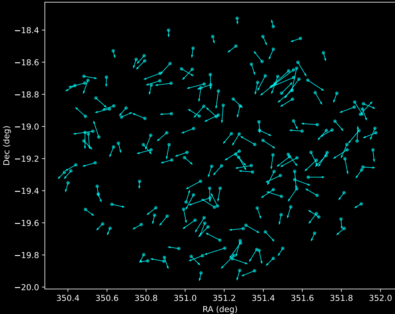
APOGEE DR17 Noise Stream Proper Motion Vectors (n=193)
